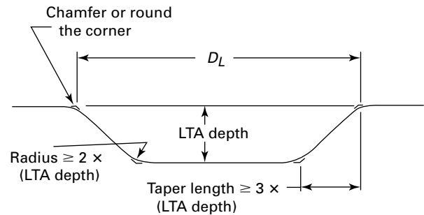
Figure IV-3-1 Blend Requirements
