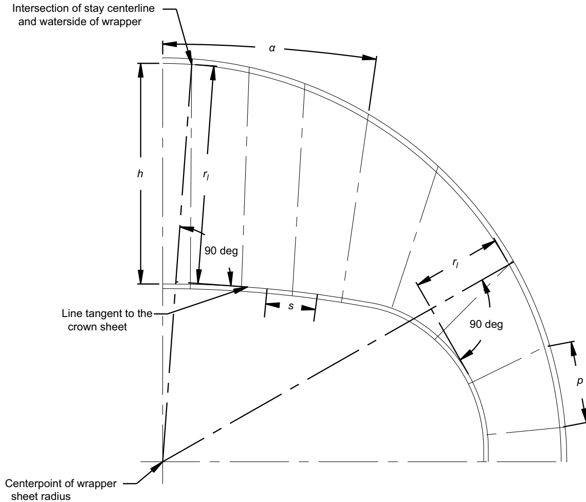
Figure PFT-23.1 Stayed Wrapper Sheet of Locomotive-Type Boiler
