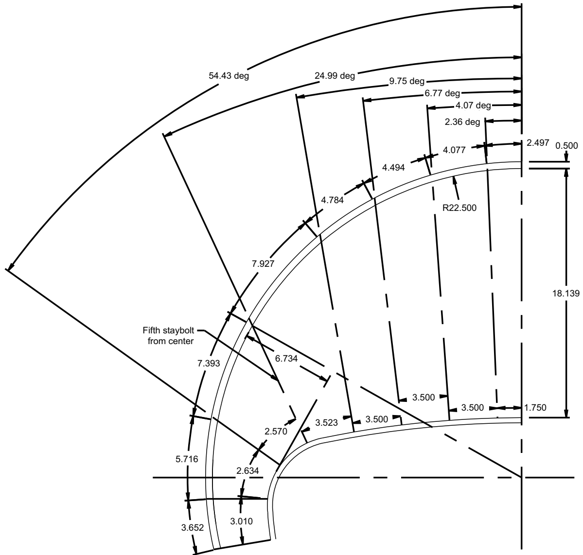
Figure A-77-1 Example of Stayed Wrapper Sheet of a Locomotive Boiler
