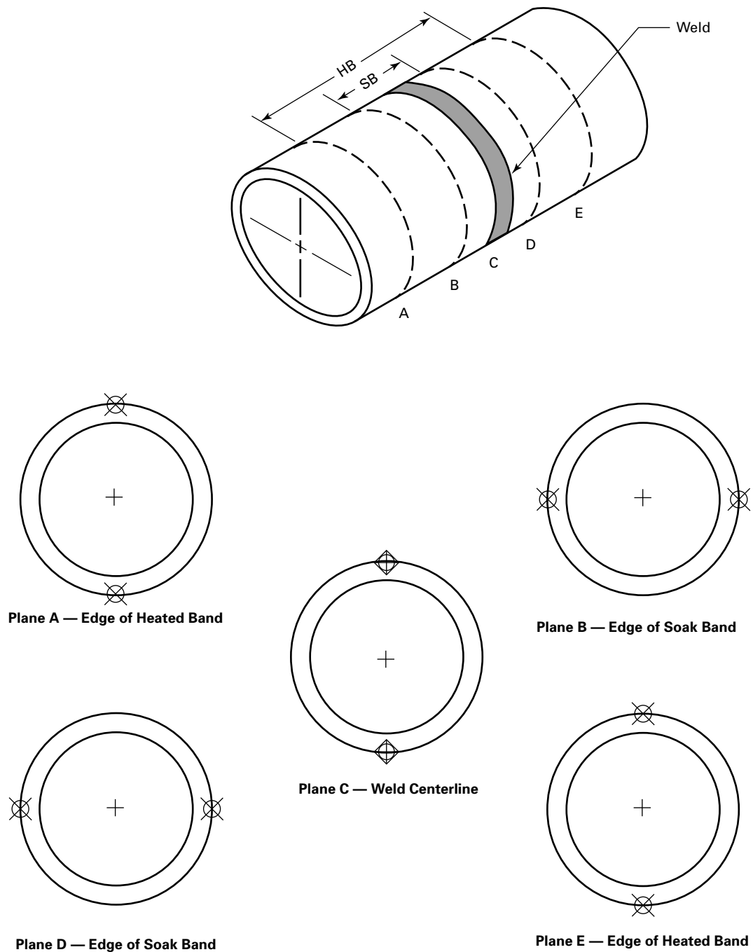
Figure VIII-6.3.4-2 Location of Thermocouples (Monitoring and Control) for Pipe Sizes NPS 6 Through NPS 12 (DN 150 Through DN 300) (25) and Two Control Zones
