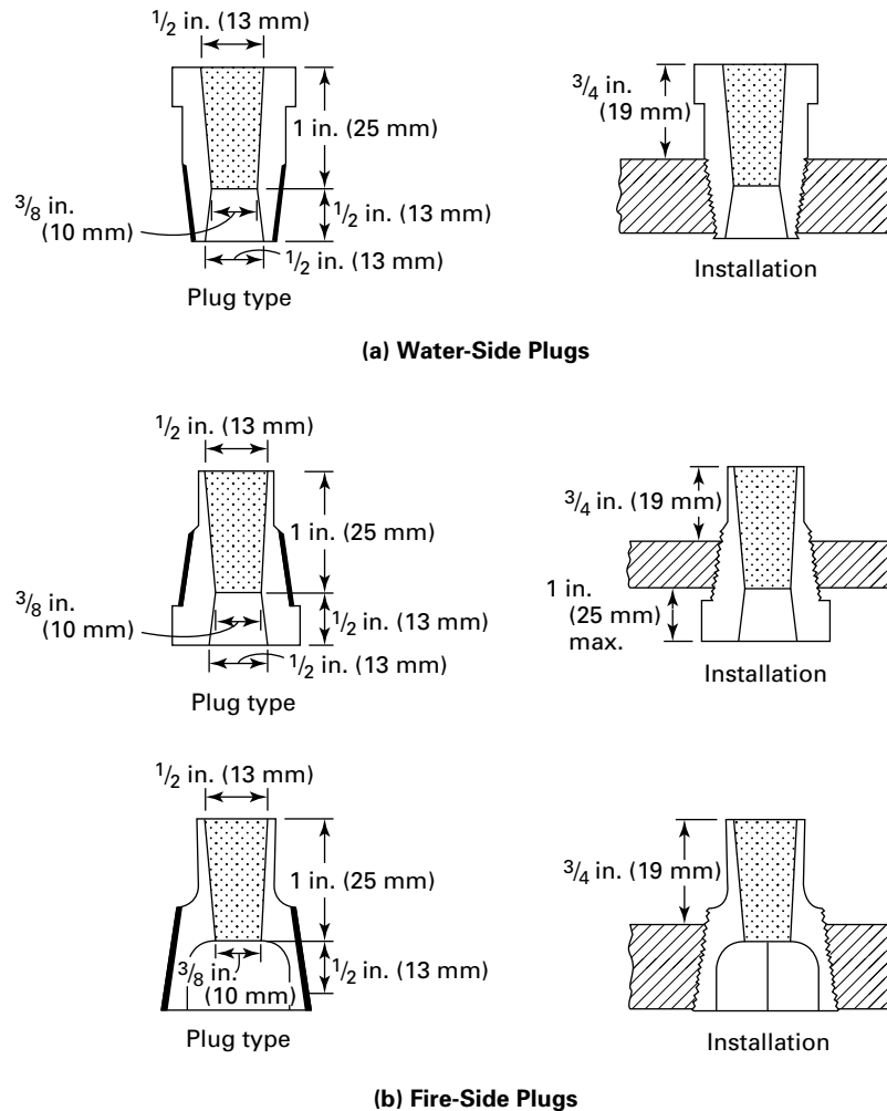
Figure A-19 Typical Forms of Fusible Plugs
