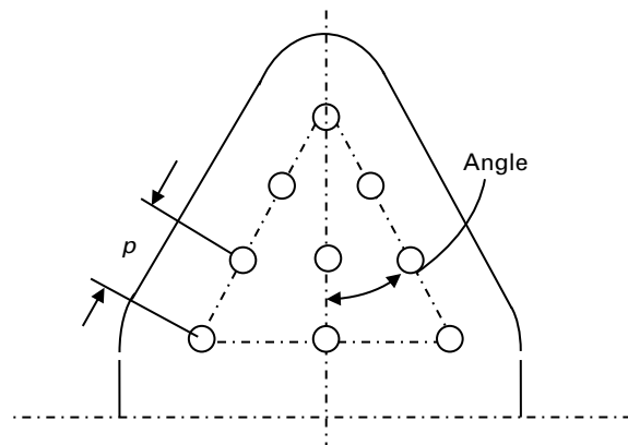
Figure PL-20.4.2-1 Diamond Riveted Plate
