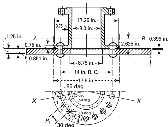
Figure A-75-1 Example of Nozzle Attached by Riveting
