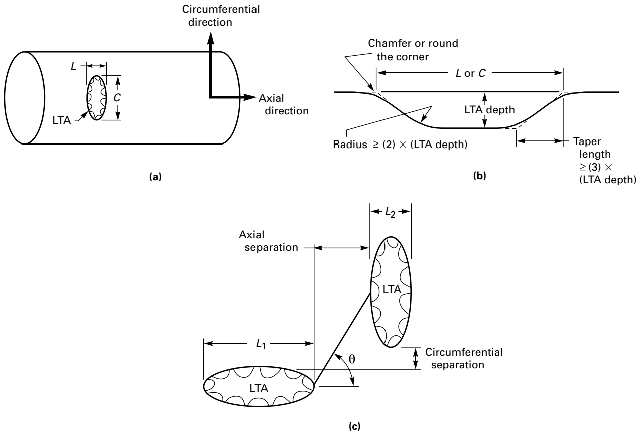
Figure IV-2-1 Symbols
