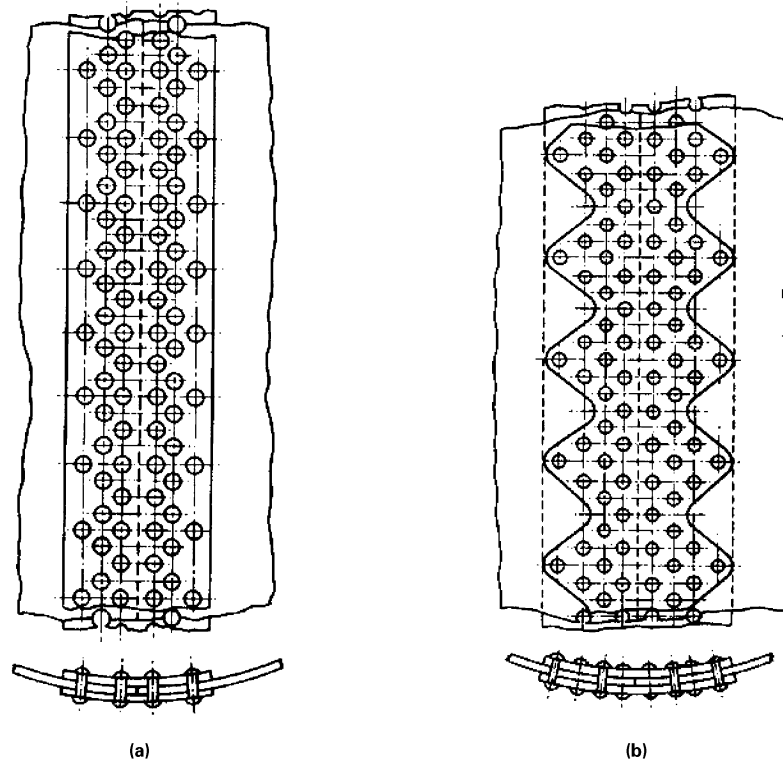
Figure A-6-2 Joints That May Be Used to Avoid Eccentric Stresses
