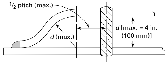
Figure PFT-20 Welding Ogee Ring
