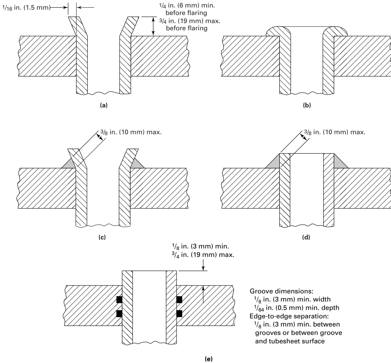
Figure PWT-11 Examples of Acceptable Forms of Tube Attachment
